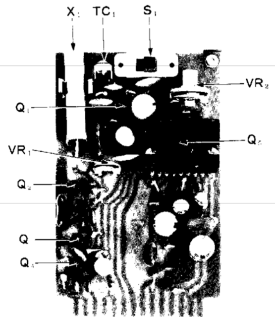
Fig. 16 AF-CALIB UNIT
